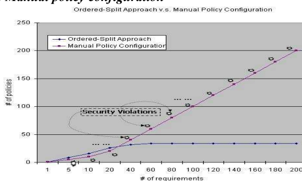
Figure 14 Ordered-Split Approach versus Manual Policy Configuration
