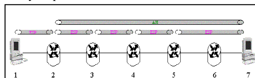
Figure 9 The solution with Ordered-Split
