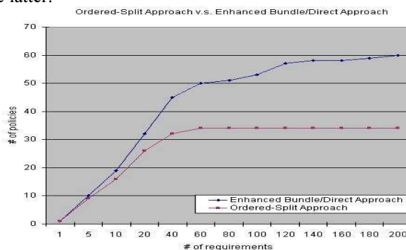
Figure 16 Ordered-Split Approach versus Enhanced Bundle/Direct Approach
