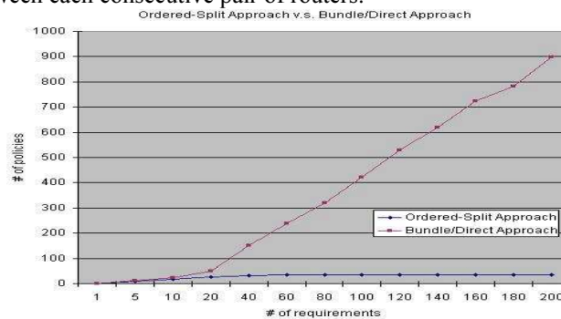
Figure 15 Ordered-Split Approach versus Bundle/Direct Approach
