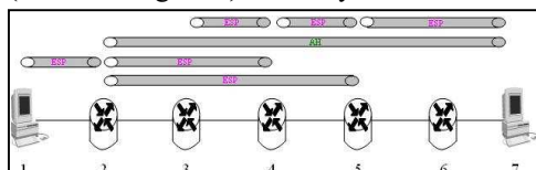
Figure 8 The solution with Direct
