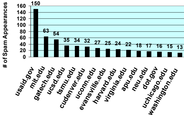
Figure 5: Layer #1: top-15 .gov/.edu domains
