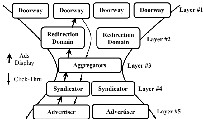
Figure 1: Spam Double-Funnel
