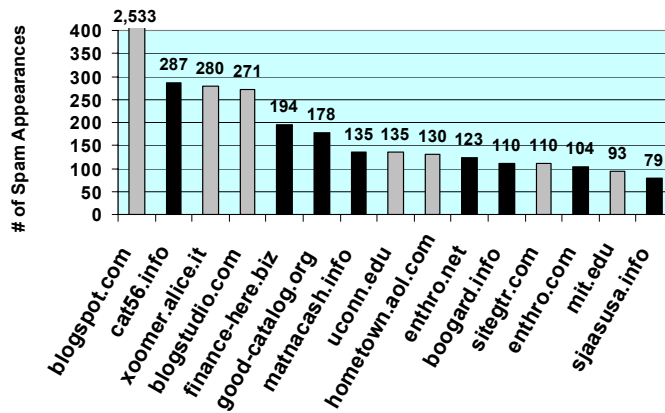
Figure 9: Layer #1: top-15 primary domains/sites by spam doorway appearance counts
